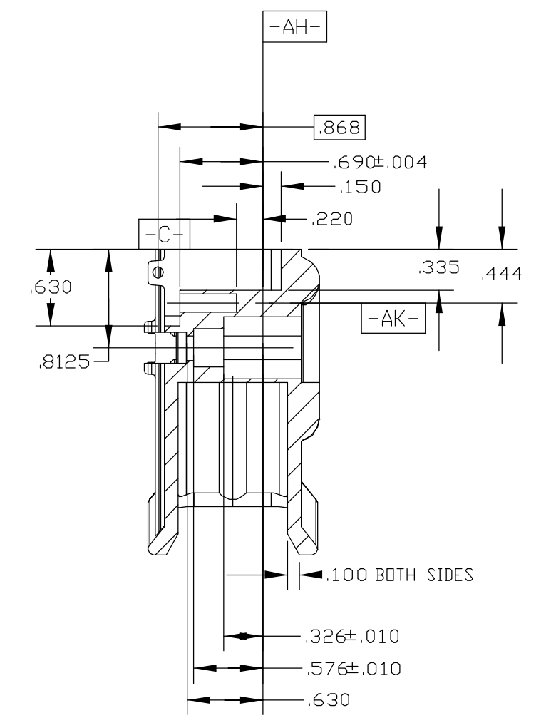
SECTION C-C
